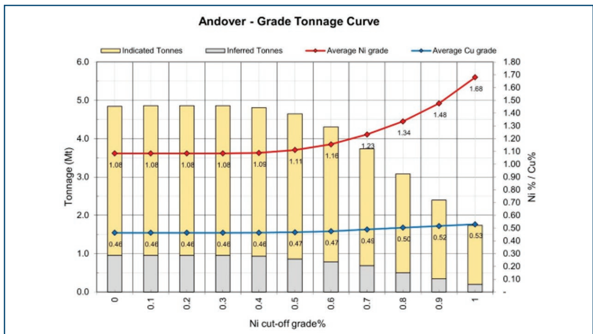
Figure 8: Andover Deposit – Grade Tonnage Curve
