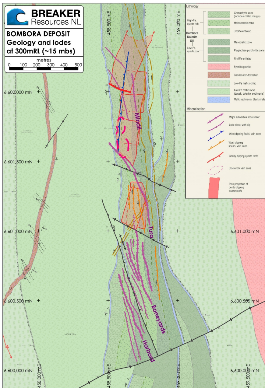
Figure 3: Bombora gold deposit geology at 300mRL (~15m below current land surface); Major steep lodes are labelled
