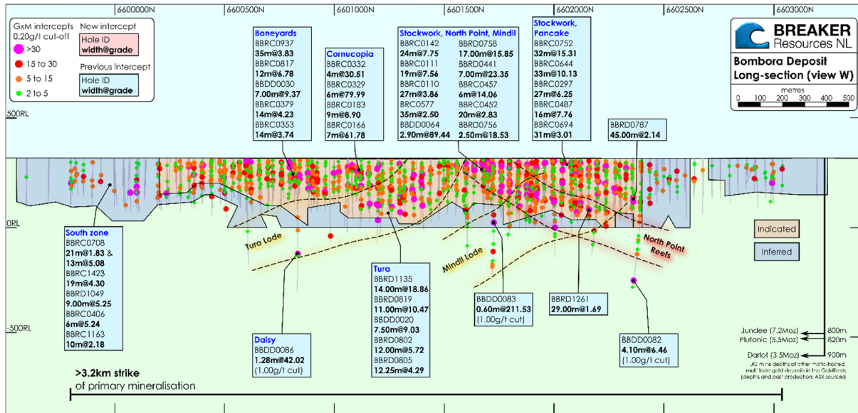
Figure 1: Long-section showing distribution of Indicated and Inferred mineralisation
