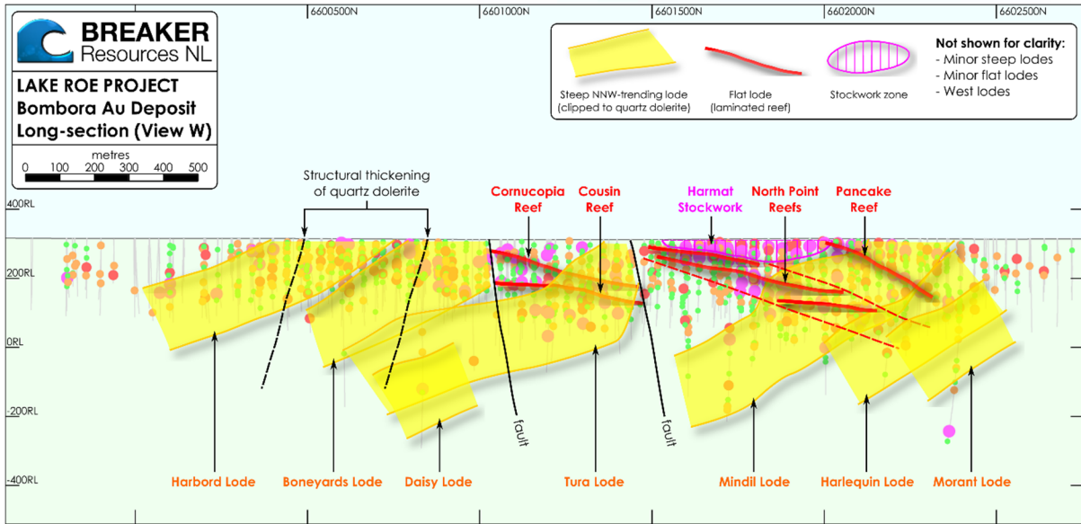
Figure 4: Long-section of the Bombora deposit, showing major steep and flat lodes. The southerly plunge of the steep lodes is caused by their intersection with the favourable quartz dolerite.
