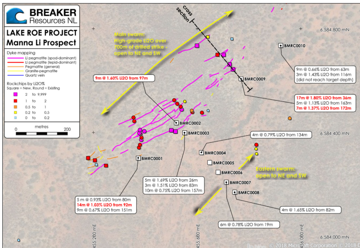
Figure 6: Plan of the spodumene-dominant zone of the Manna Lithium Prospect, showing the maiden RC drilling collars and results, plus surface mapping and rock chip information
