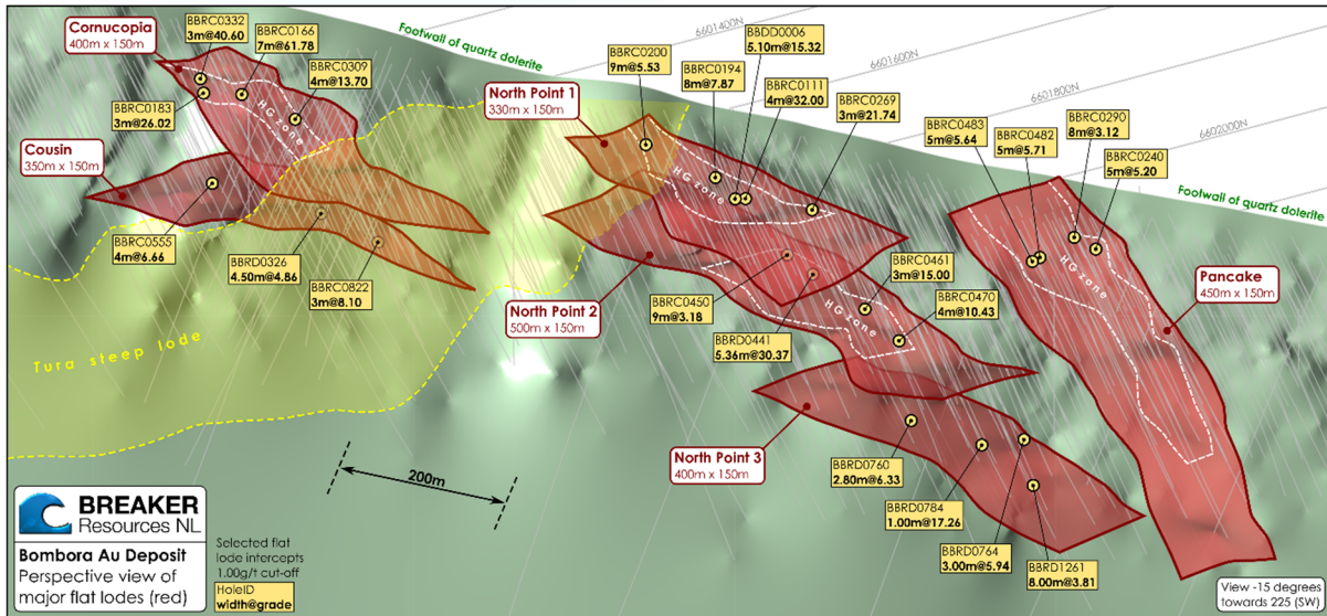
Figure 5: Perspective view of major flat lodes in relation to Tura lode (looking southwest)
