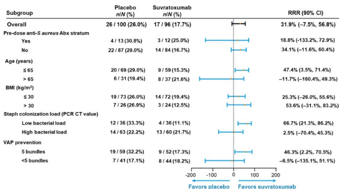
Figure 1. Results of Pre-Specified Subgroup Analyses
