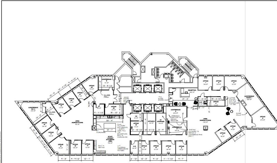
TREVI- OPTION 2A PROPOSED FLOOR PLAN SCALE: 1/8" = 1'-0"
