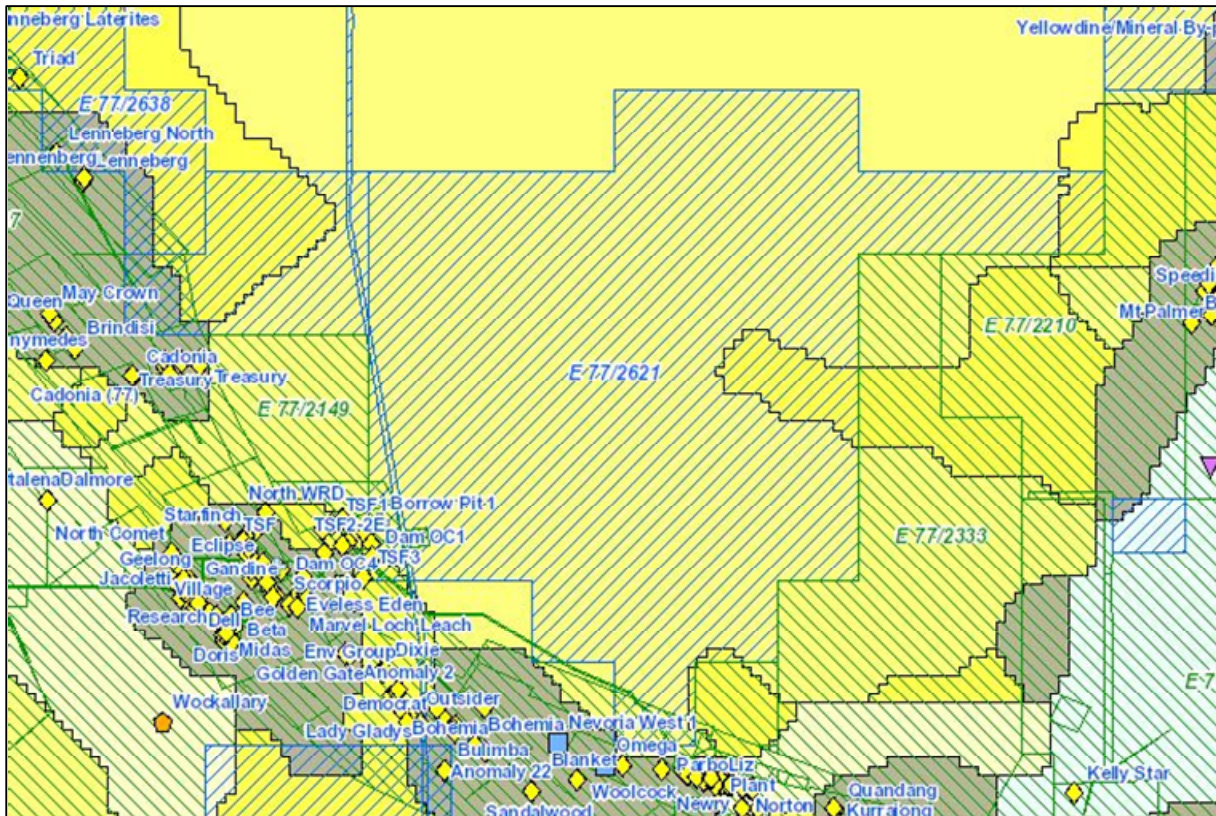
Airfield Project showing the GSWA Regolith map
