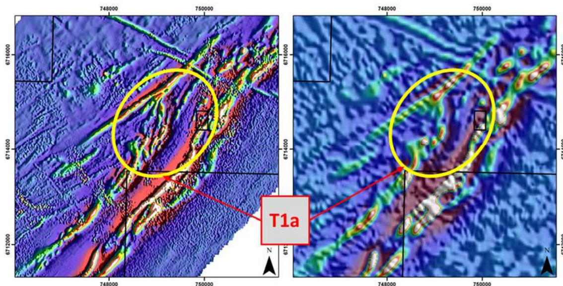
Figure 12: T1a Prospect – detailed magnetic survey (left) vs regional magnetic survey (right)
