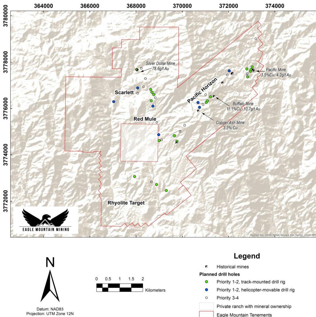
Figure 7 - Drill program showing drill locations and priority
