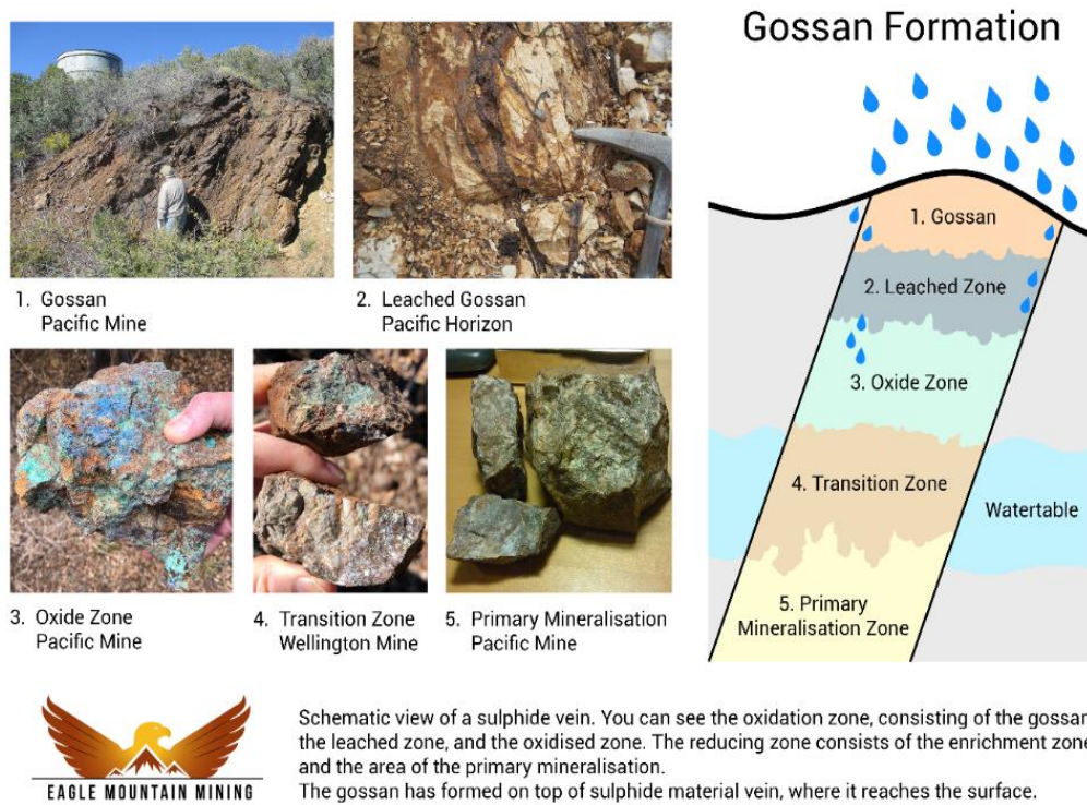
Figure 5 - Schematic of gossan development
