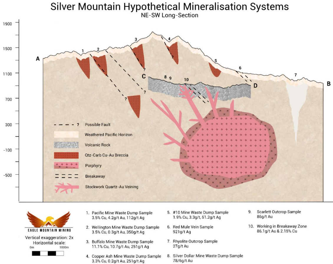
Figure 4 - Styles of mineralisation identified at Silver Mountain
