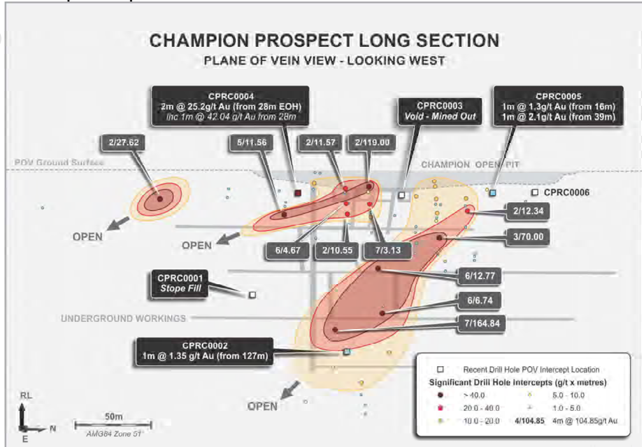
Figure Five – Champion Plane of Vein Section with recent drilling.
