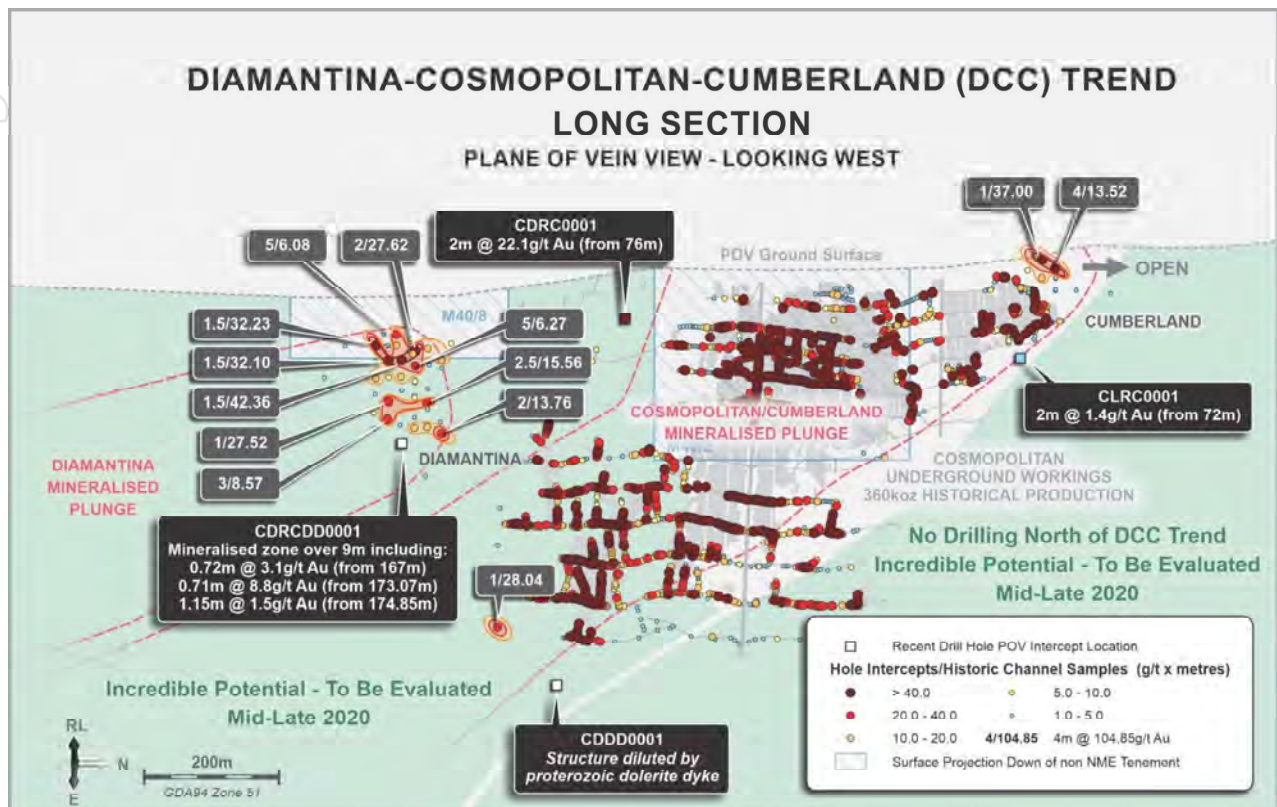
Figure Four – Cosmopolitan Gold Mine Long Section with Underground Workings with Channel Samples illustrated as gram metres*.
