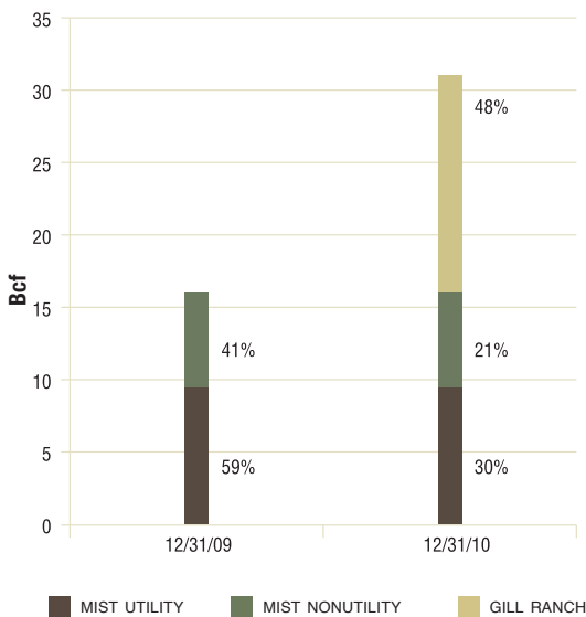
GAS STORAGE CAPACITY (working gas capacity)
