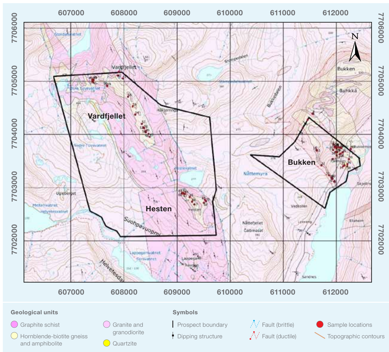
Geological map and sample locations at Hesten and Vardfjellet (left), and Bukken (right) prospects in Senja.
