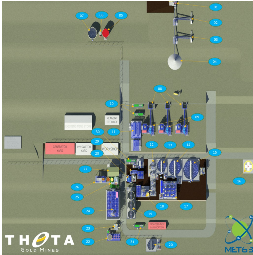
Figure 12: New TGME Plant Layout
