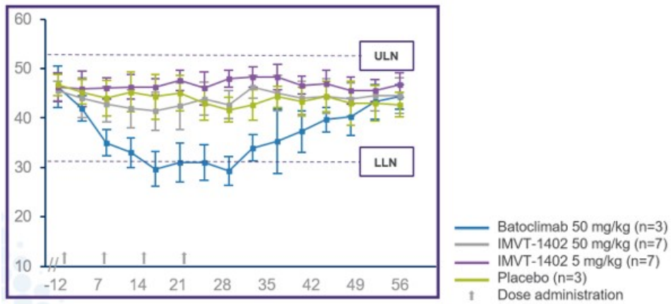
Mean Change in Albumin in Head-to-Head Study of IMVT-1402 and Batoclimab in Cynomolgus Monkey
