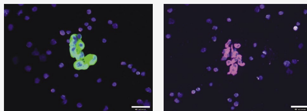
Example images of epithelial and mesenchymal staining in CTCs using the Portrait Flex assay.
