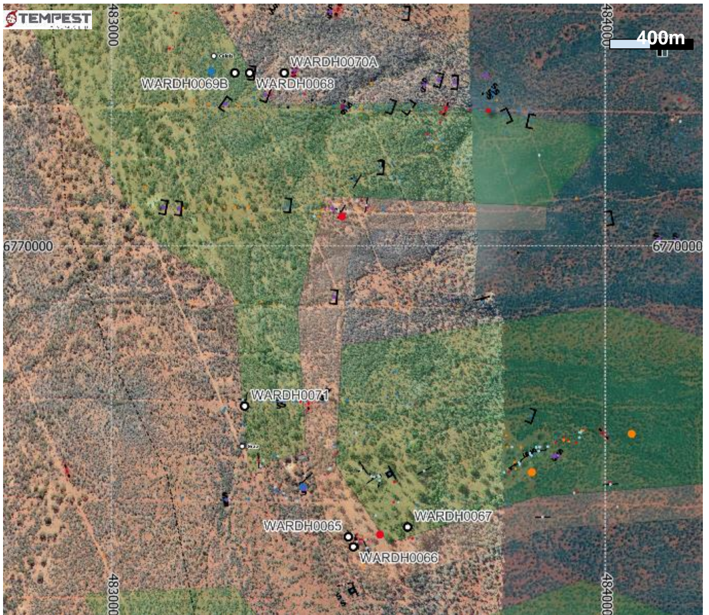
Figure 11: Geological mapping of the drilling area
