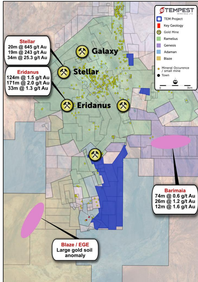
Figure 17: Range Project tenure (blue) with regional neighbours
