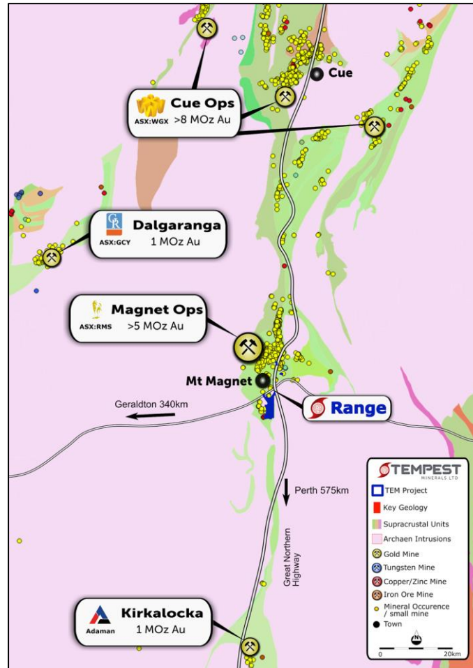
Figure 16: Stylised Mt Magnet regional geology map
