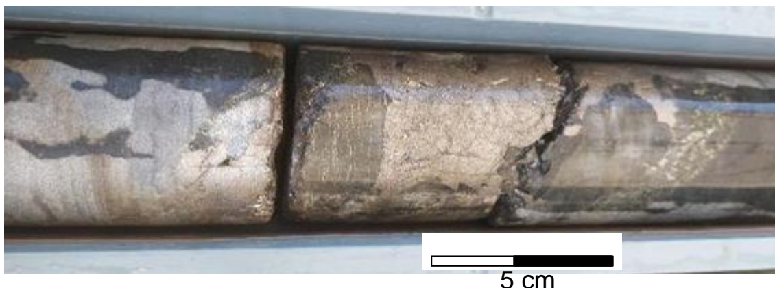
Figure 10: Pyrrhotite and chalcopryite vein WARDH0068 (164.10m)
