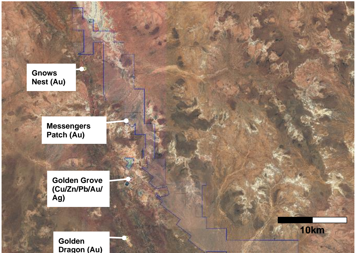
Figure 15: Overview of Messenger Project tenements
