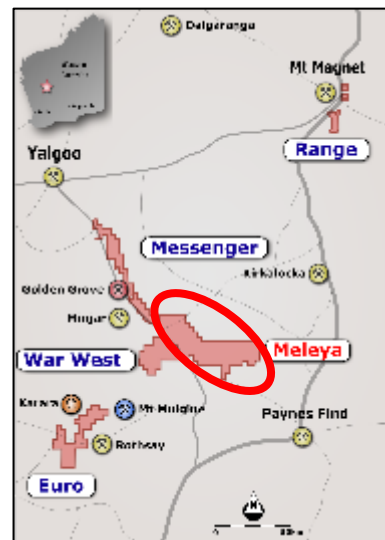
Figure 3: Meleya Project Location
