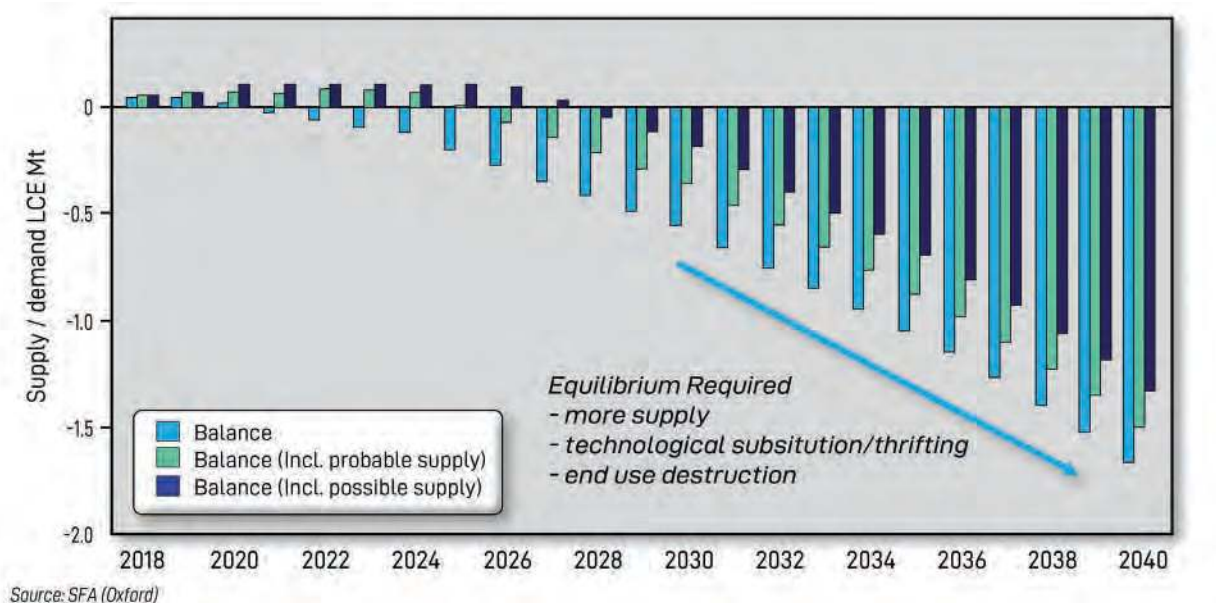
Figure 2 – Projected lithium market supply/demand
