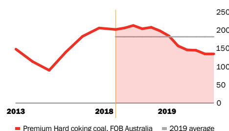
Coal, US$/t
