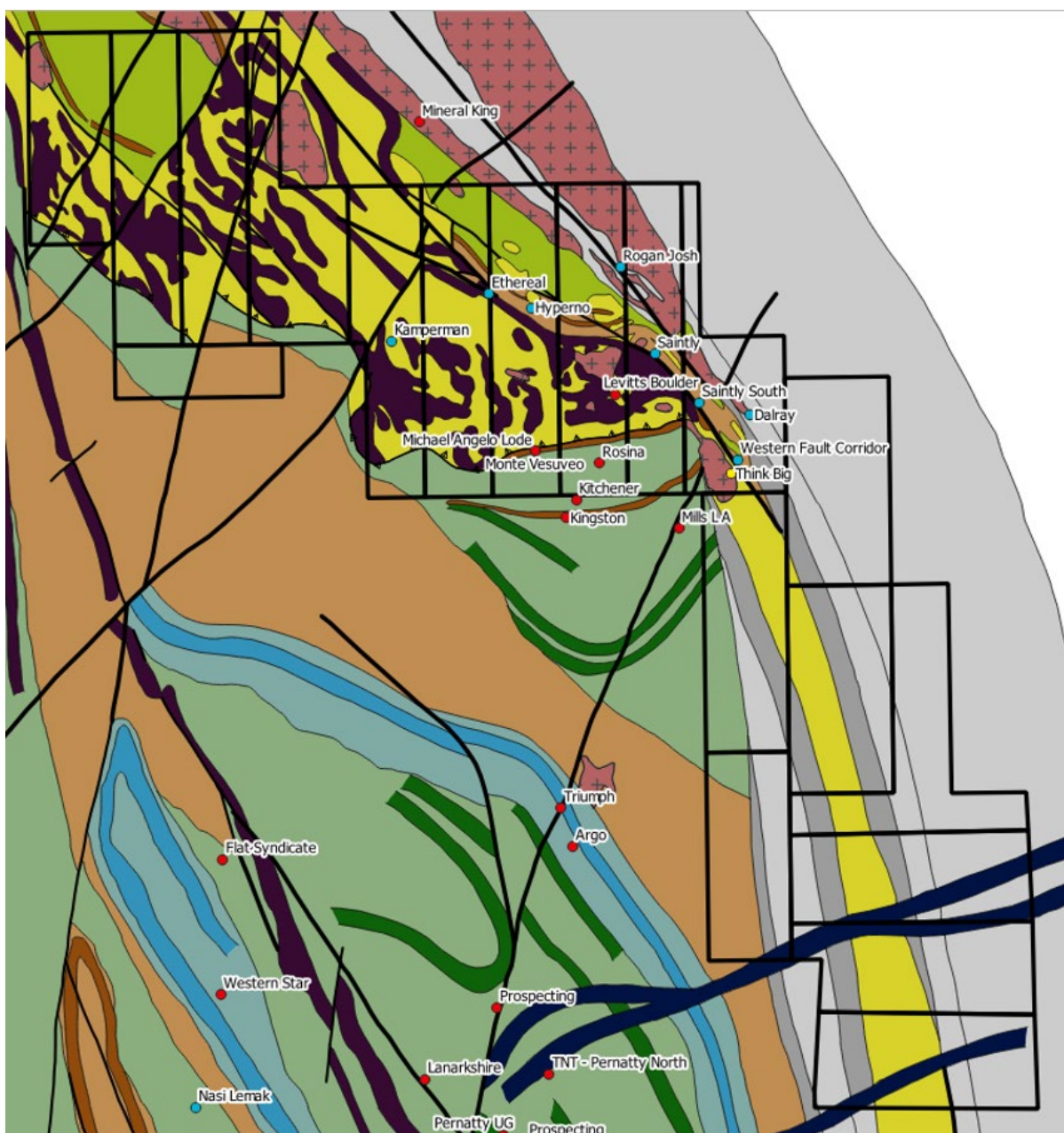
Figure 10 – Feysville local area geology
