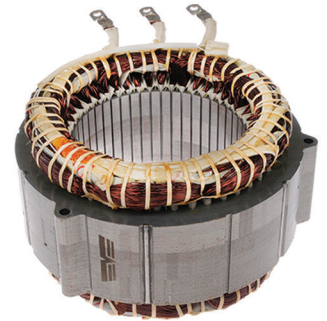
Prius Transmission Stator
