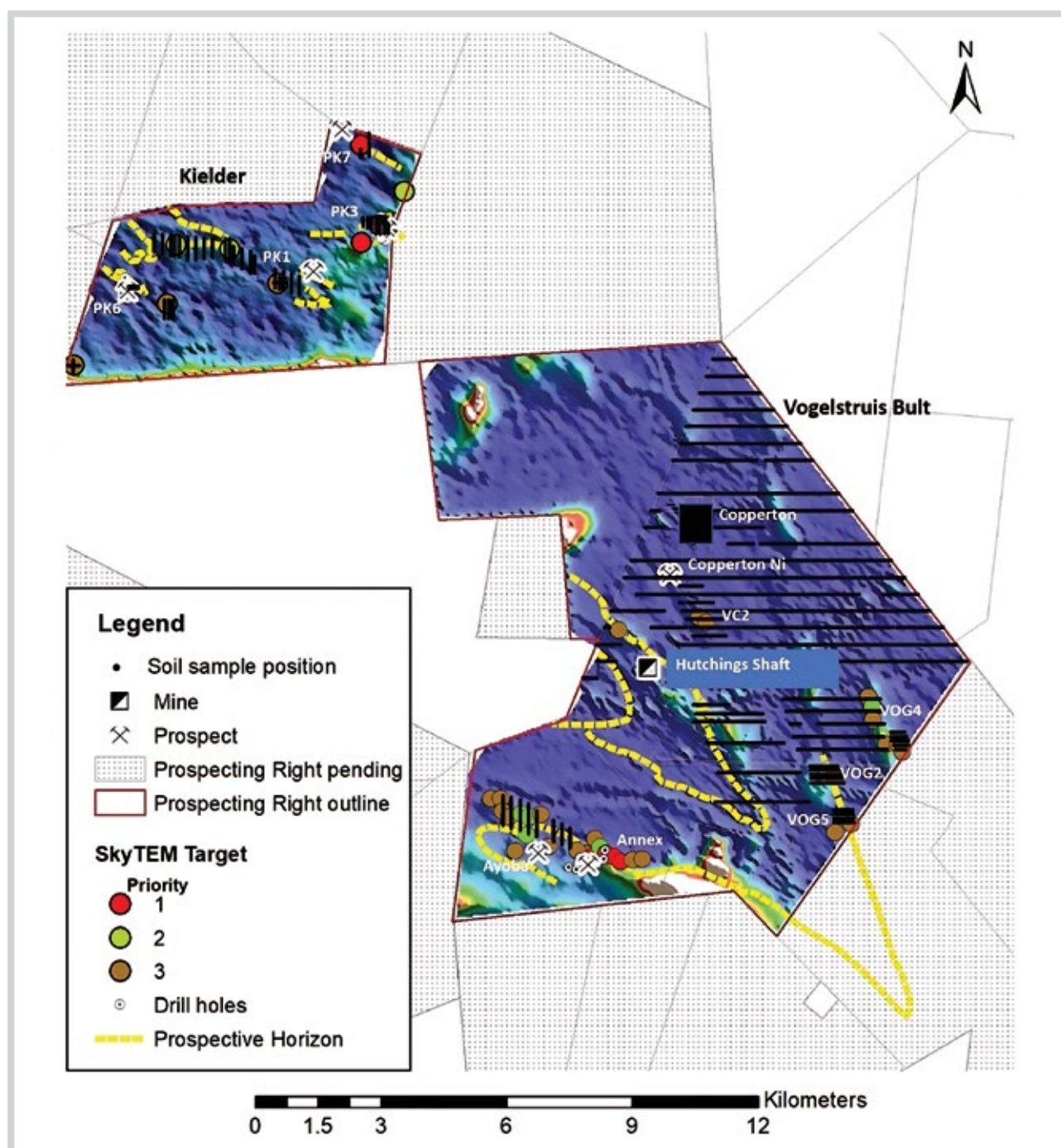
Figure 12: Channel 25 SkyTEM™ image showing soil sampling completed to date.
