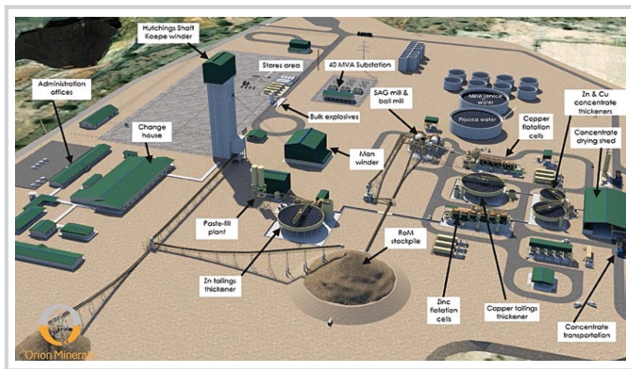
Figure 5: General surface, shaft and plant layout.
