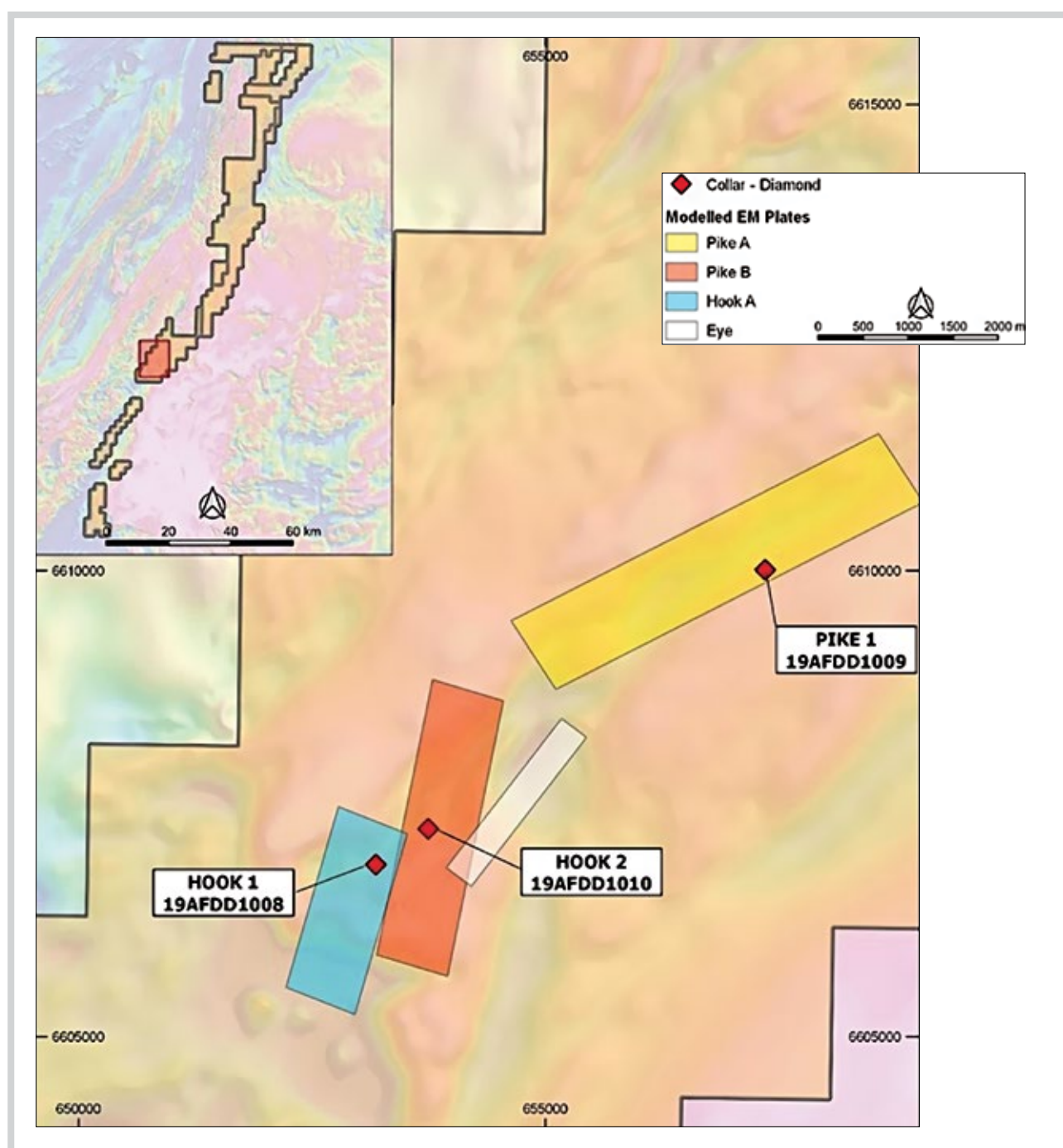
Figure 22: Plan view of the Pike 1, Hook 1 and 2 prospects with diamond drill holes and targeted conductors plotted on airborne magnetics.
