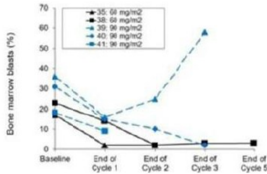
Figure 4. Five out of six patients in cohorts 7 and 8 receiving the combination prexigebersen + LDAC have greater than 50% decrease in bone marrow blasts
