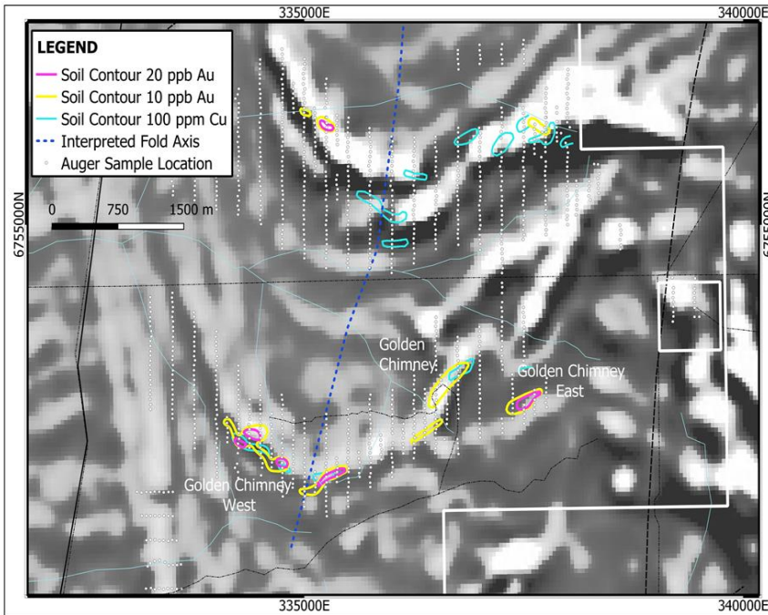
Figure 14. Multi-element (Au, Cu) soil contours derived from Shree’s auger program. Also illustrated is the location of all auger samples and the interpreted position of the regional fold axis. The underlying image is the aerial magnetics.
