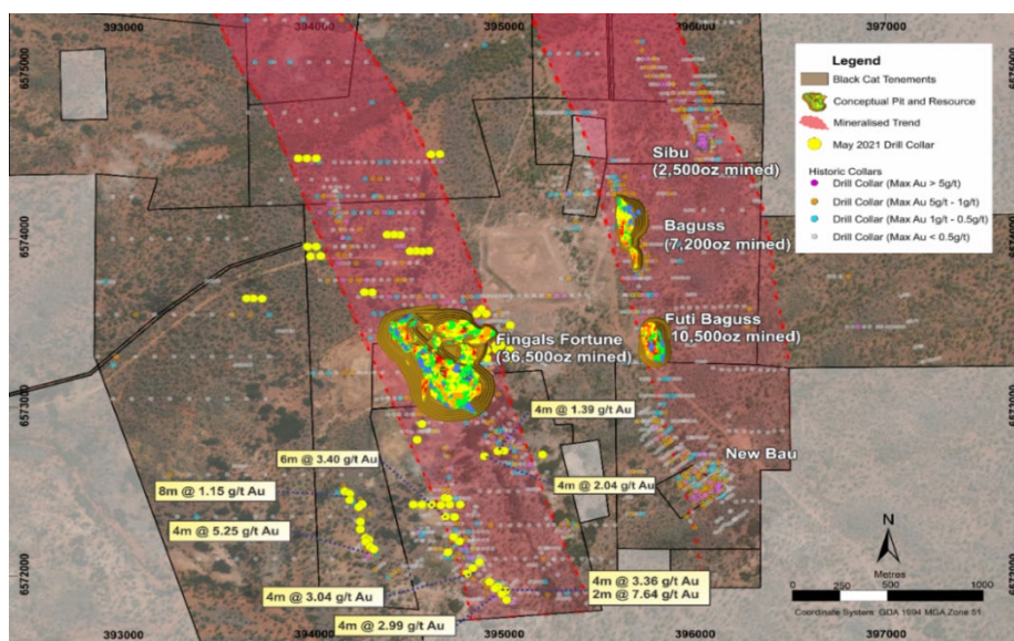
Figure 6: Plan view of Fingals Mining Centre with recent regional drilling and Resources over conceptual pit design
