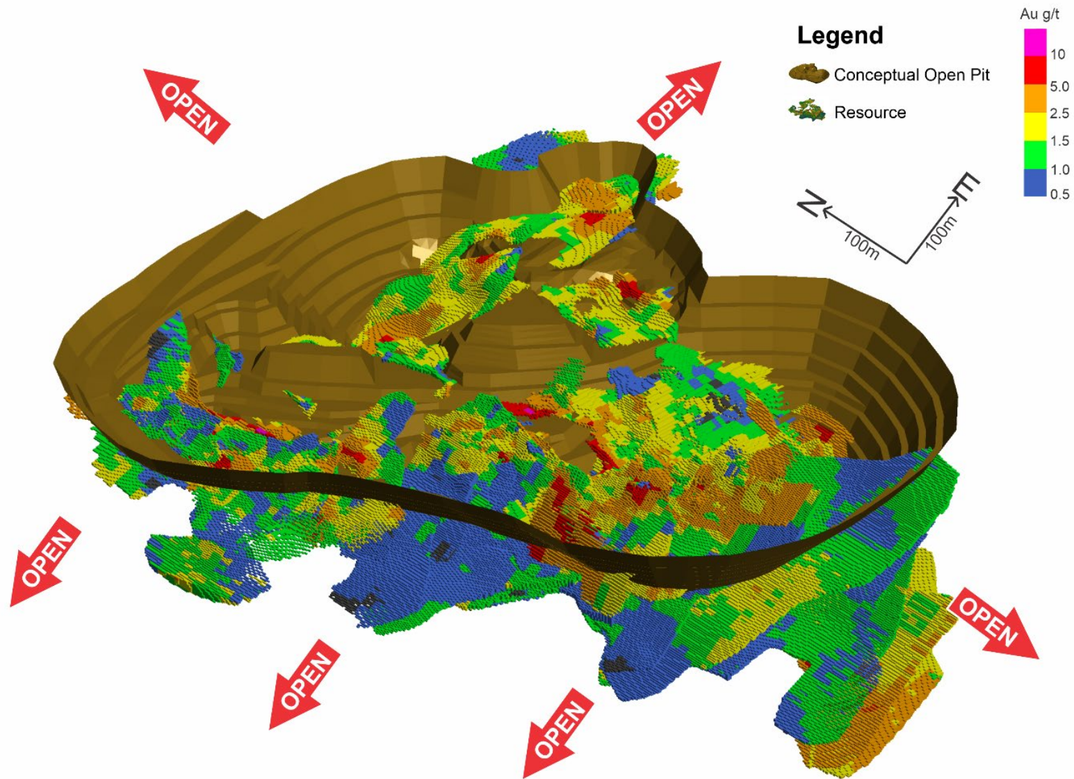
Figure 8: Conceptual pit design at Fingals Fortune with Resource, which remains open in all directions and at depth
