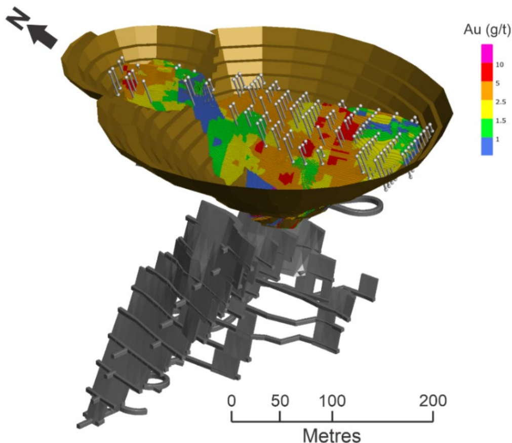
Figure 9: Conceptual open pit and underground at Myhree with Resource contained within the pit coloured by Au. Completed grade control displayed as grey lines
